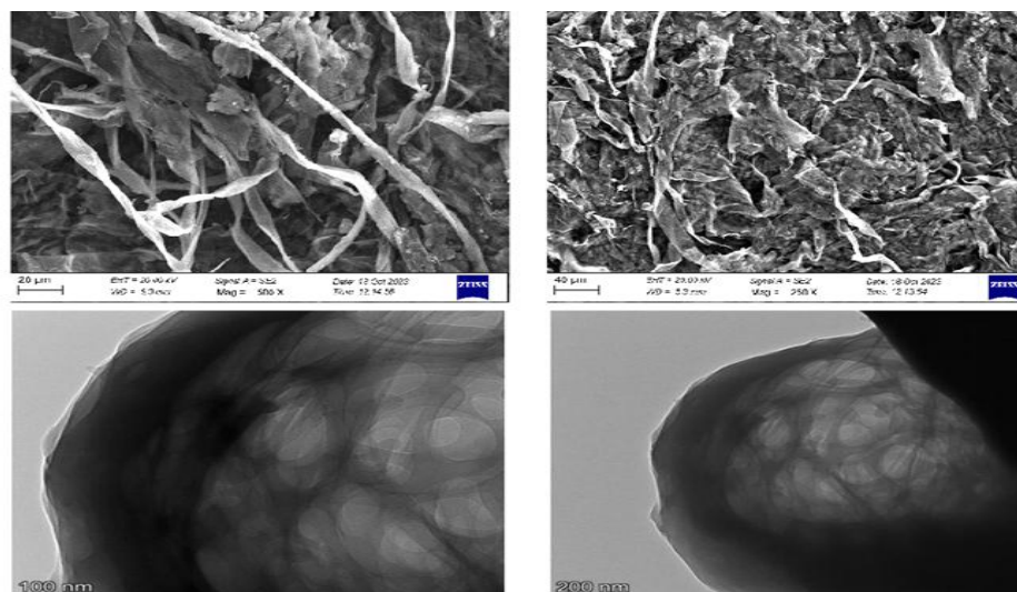
Figure 2. SEM, TEM analysis of WH nanocellulose
