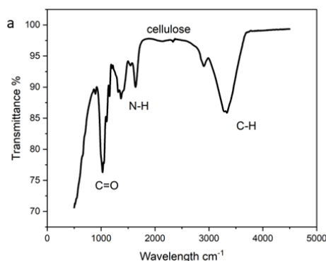
Figure 3. Give separate figure number for FTIR analysis of WH nanocellulose
