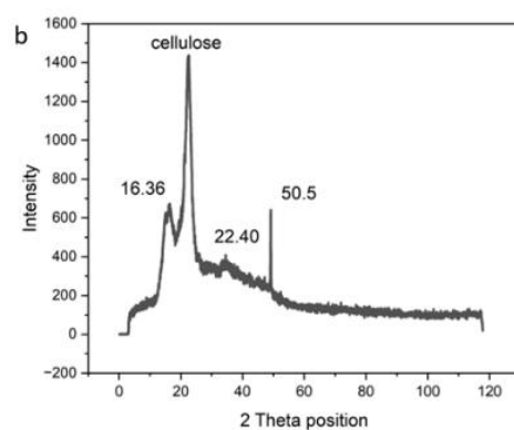
Figure 4. XRD analysis of WH nanocellulose
