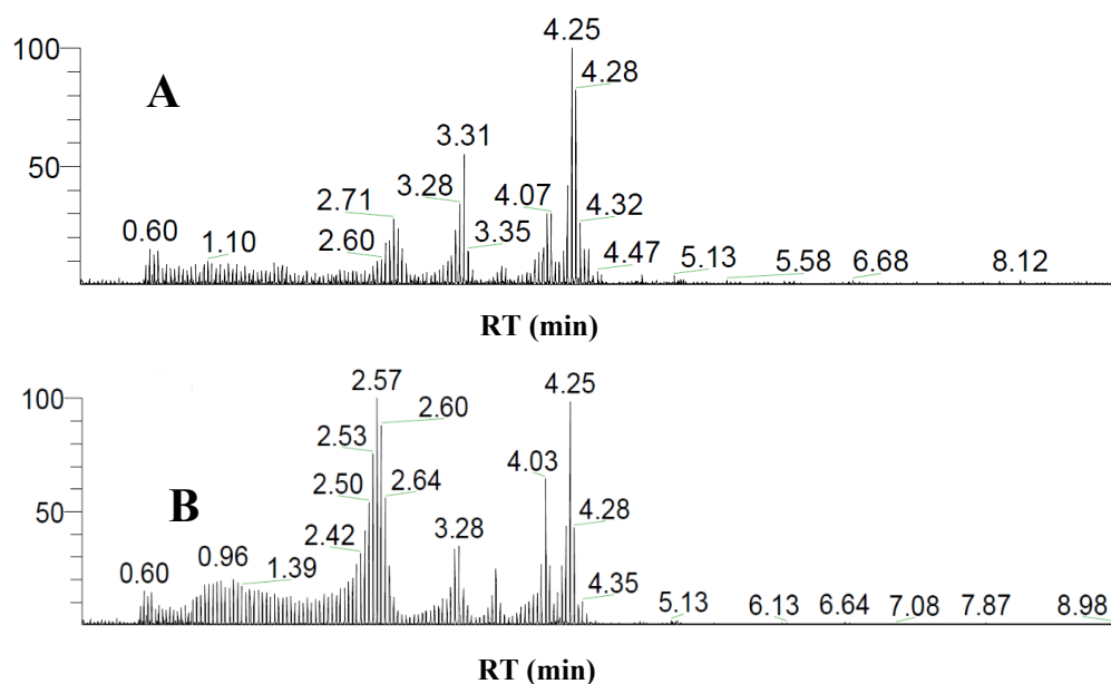
Figure 2. The MS profile of clove flower related to flavonol constituents. A. FS-1 (at 4 months); B. F-4 (at 7.5 months). RT. 3.28 min= Luteolin-7- O -glycoside; RT. 5.13 min = Myricetin; RT. 3.03 min = Myricetin-3- O -glycoside; RT. 6.64 min = Apigenin-7- O -glycoside; RT. 4.20 min = Quercetin; Rt. 4.25 min = Quercetin-3- O -glycoside
